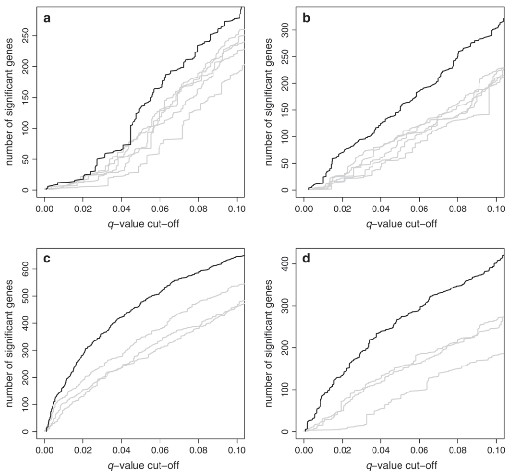
Fig. 3. A comparison of the ODP approach to five leading methods for identifying differentially expressed genes (described in the text and Figure 2) based on simulated data. The number of genes found to be significant by each method over a range of estimated q -value cutoffs is shown for a single, representative data set from each scenario. The proposed ODP approach is in black and the other methods are in gray. In general, the data sets increase in complexity from panels (a) to (d). (a) In this scenario, two groups are compared, there is perfectly symmetric differential expression, and the variances are simulated from a unimodal, well-behaved distribution. (b) Two groups are compared, there is moderate asymmetry in the differential expression, and the variances are simulated from a bimodal distribution. (c) Three groups are compared, there is slight asymmetry in differential expression, and the variances are simulated from a unimodal, well-behaved distribution. (d) Three groups are compared, there is moderate asymmetry in differential expression, and the variances are simulated from a bimodal distribution.
