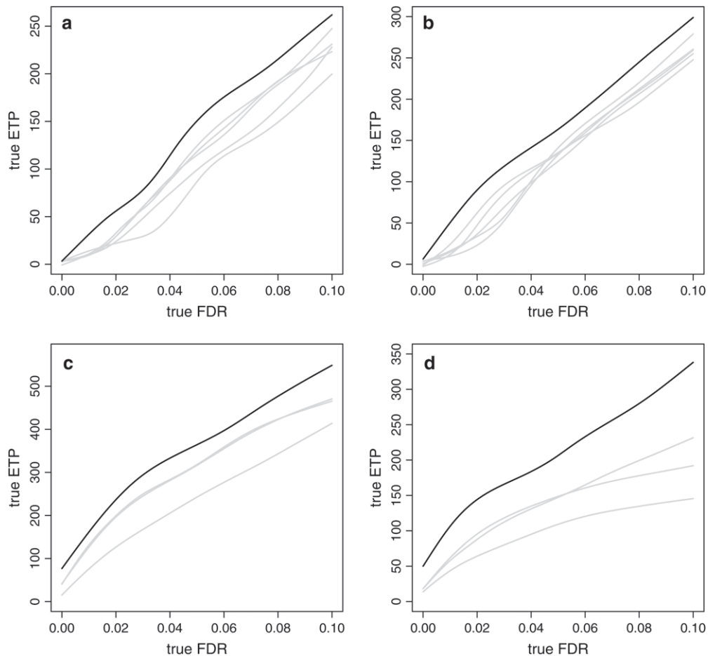
Fig. 4. A comparison of the ODP approach to five leading methods for identifying differentially expressed genes (described in the text and Figure 2) based on simulated data. The ETP genes is shown for each true FDR level. As opposed to Figure 3, we have averaged over 100 data sets here and taken into account knowledge of which genes are true and false discoveries in order to make these exact calculations. Panels (a), (b), (c), and (d) are analogous to those in Figure 3.
